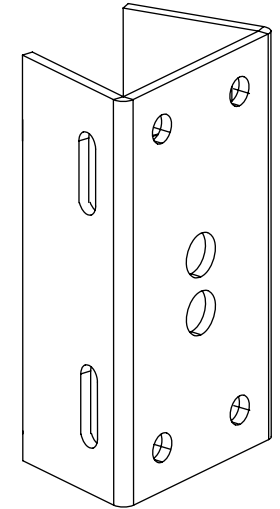
A (1) Aluminum Corner Bracket
